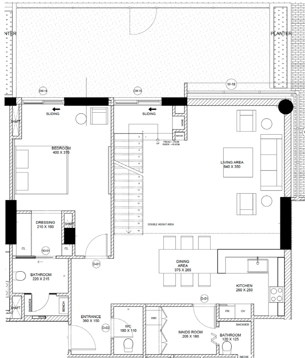
Lower Floor
