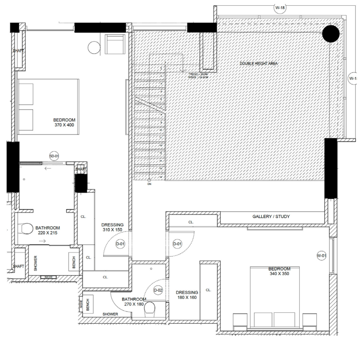
Upper Floor
