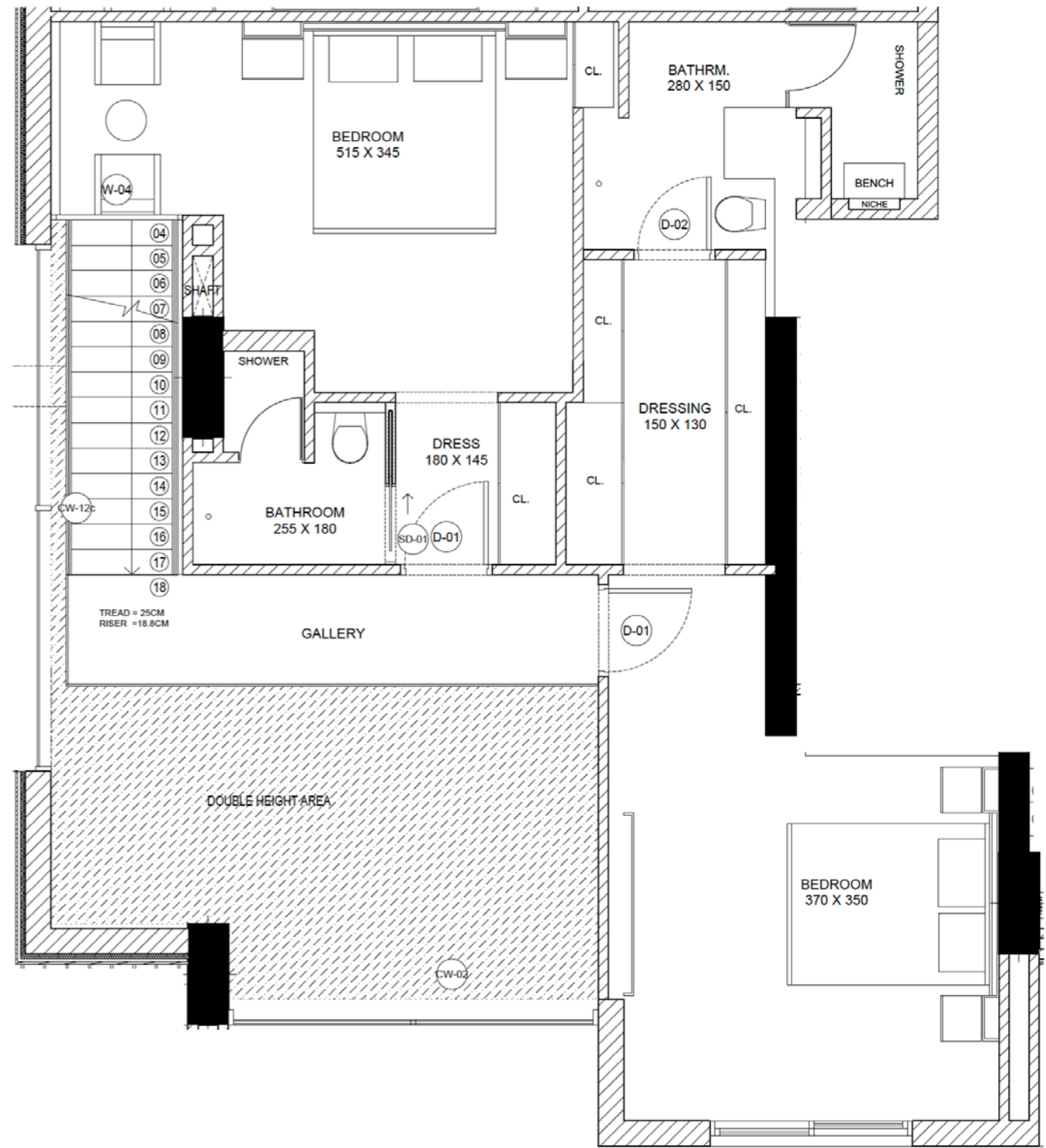
Upper Floor
