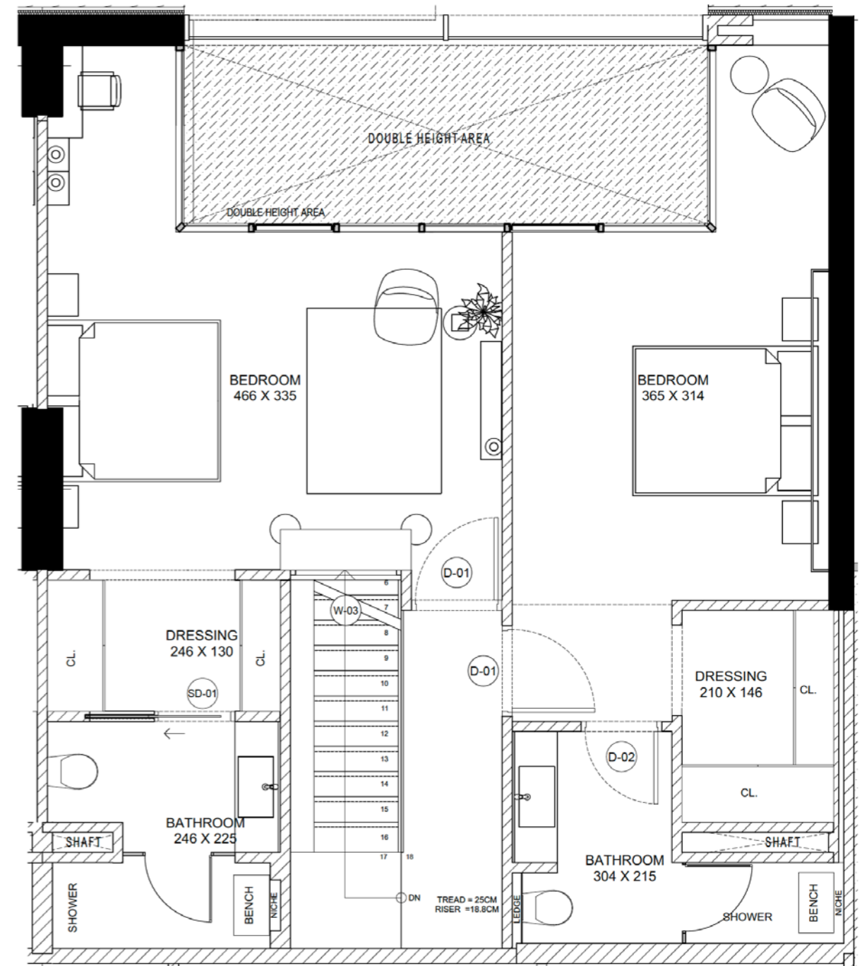
Upper Floor
