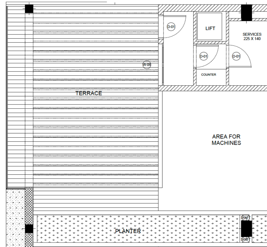
Roof Terrace
