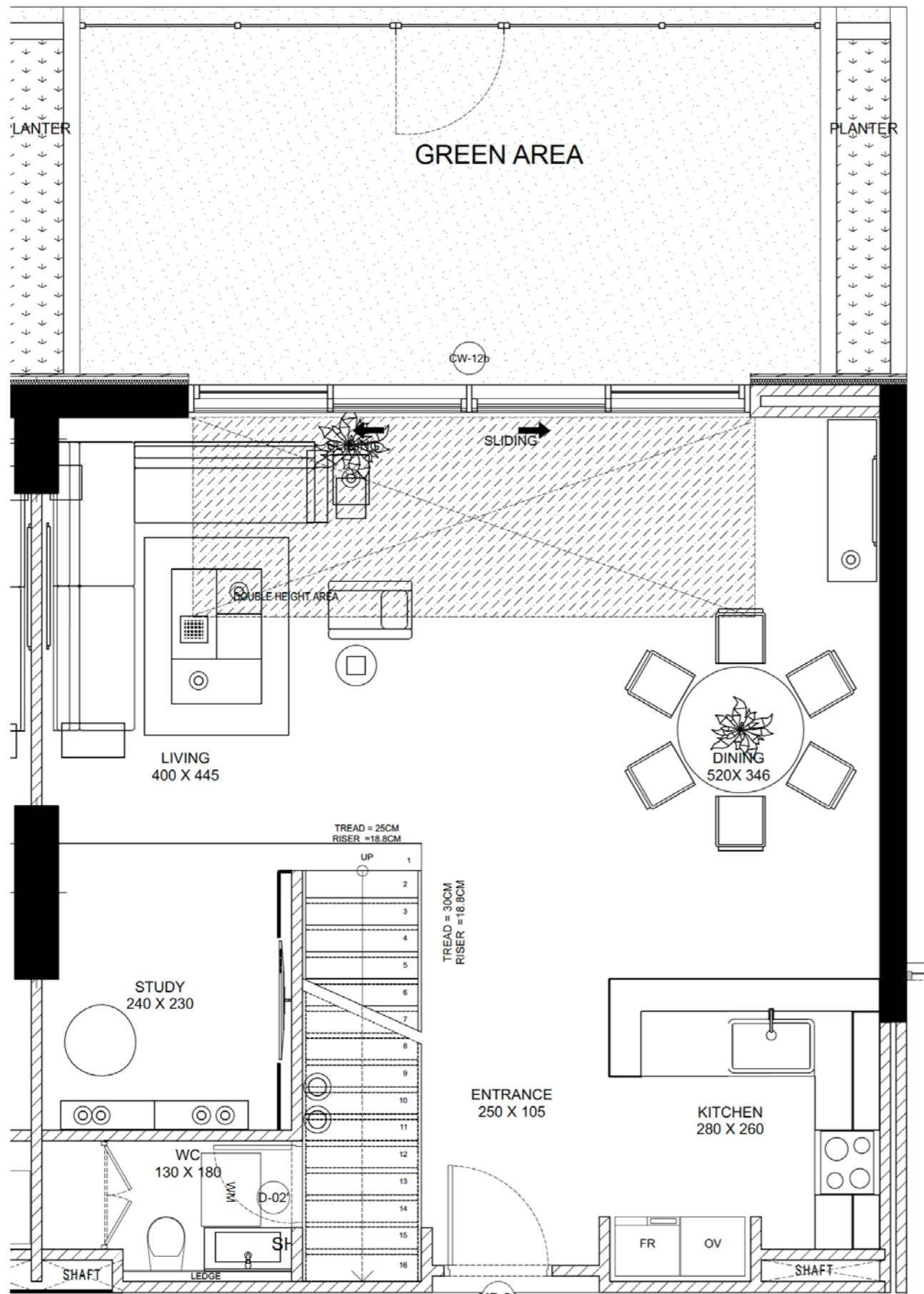
Lower Floor
