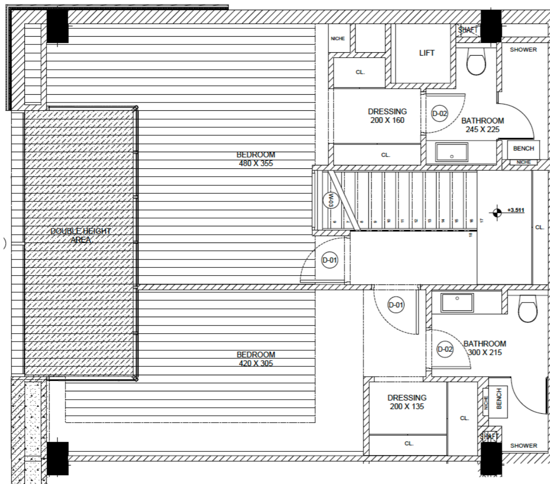
Upper Floor
