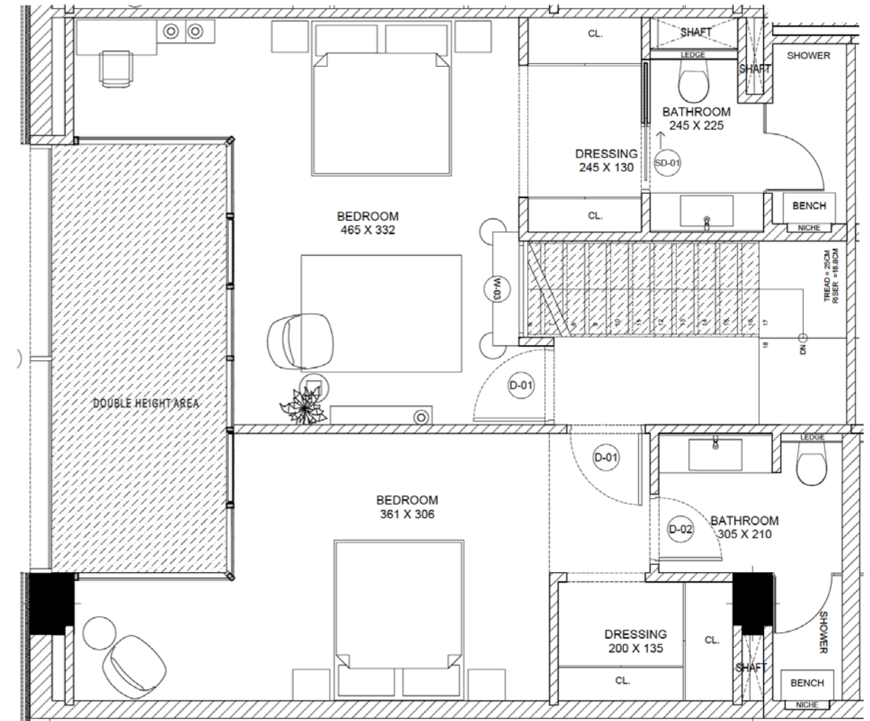
Upper Floor
