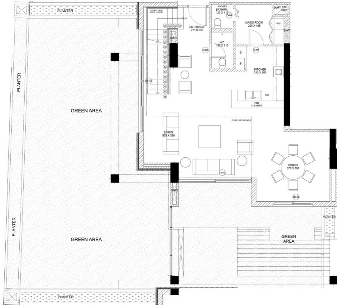
Lower Floor
