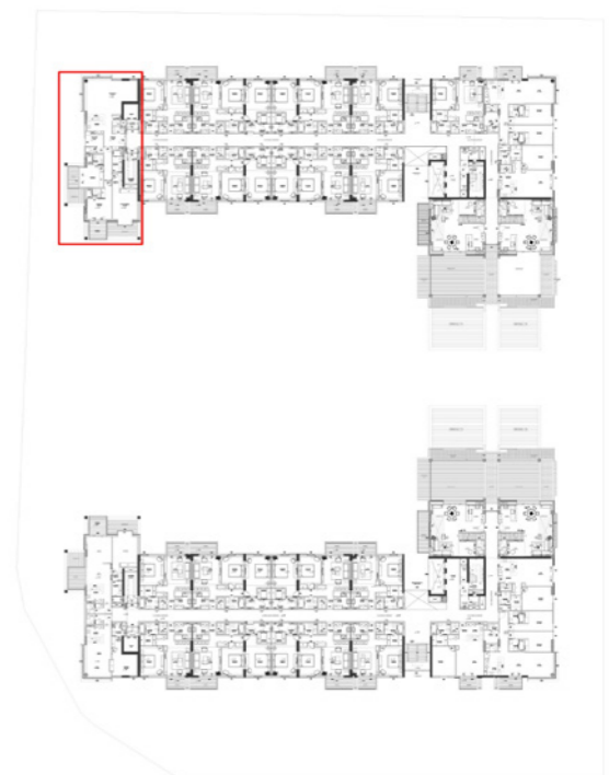
Fourth Floor
